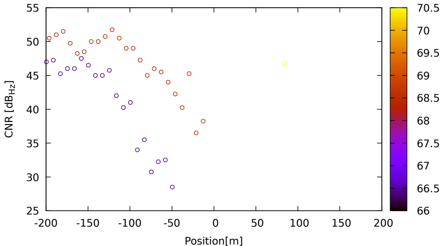
CNR vs position for G03 (L2) on LeicaGS15 - DOY 262 jam. 2
