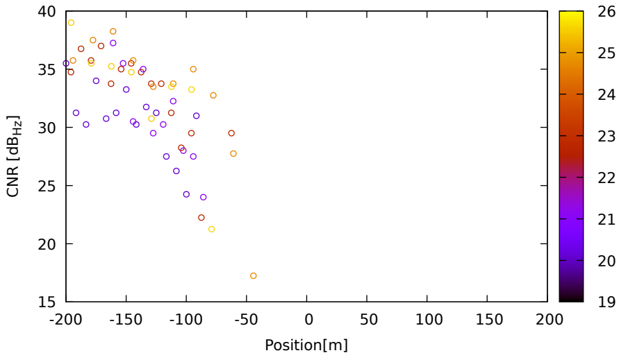
CNR vs position for G04 (L2) on LeicaGS15 - DOY 262 jam. 1
