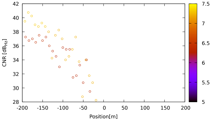
CNR vs position for G08 (L2) on LeicaGS15 - DOY 262 jam. 3
