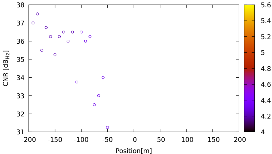
CNR vs position for G09 (L2) on LeicaGS15 - DOY 262 jam. 3
