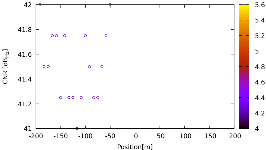
CNR vs position for G09 (L5) on LeicaGS15 - DOY 262 jam. 3
