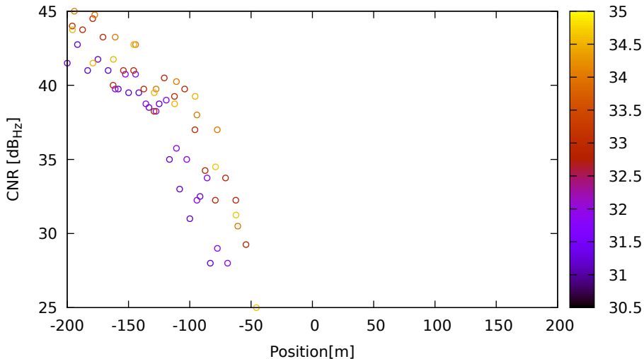
CNR vs position for G17 (L2) on LeicaGS15 - DOY 262 jam. 1
