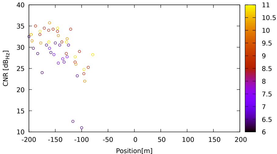
CNR vs position for G19 (L2) on LeicaGS15 - DOY 262 jam. 1
