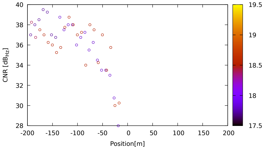
CNR vs position for G19 (L2) on LeicaGS15 - DOY 262 jam. 3
