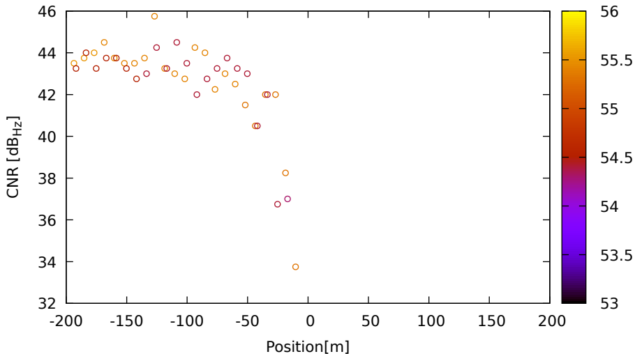
CNR vs position for G21 (L2) on LeicaGS15 - DOY 262 jam. 3
