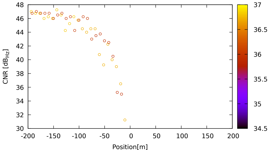
CNR vs position for G22 (L1) on LeicaGS15 - DOY 262 jam. 3
