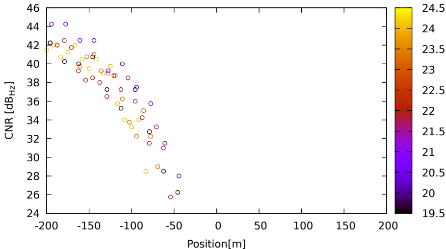
CNR vs position for G32 (L1) on LeicaGS15 - DOY 262 jam. 1
