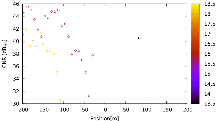
CNR vs position for G32 (L2) on LeicaGS15 - DOY 262 jam. 2
