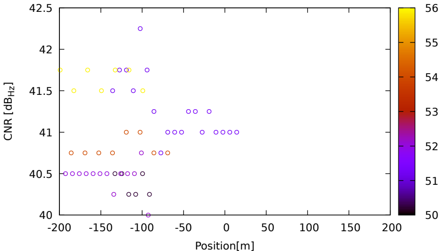
CNR vs position for R01 (G2) on LeicaGS15 - DOY 262 jam. 2
