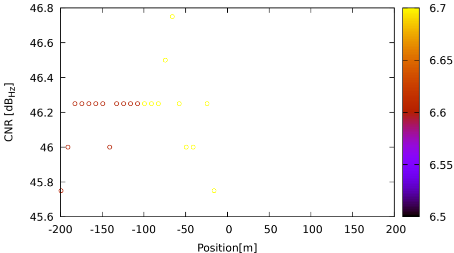
CNR vs position for E03 (E5b) on LeicaGS15 - DOY 262 jam. 3
