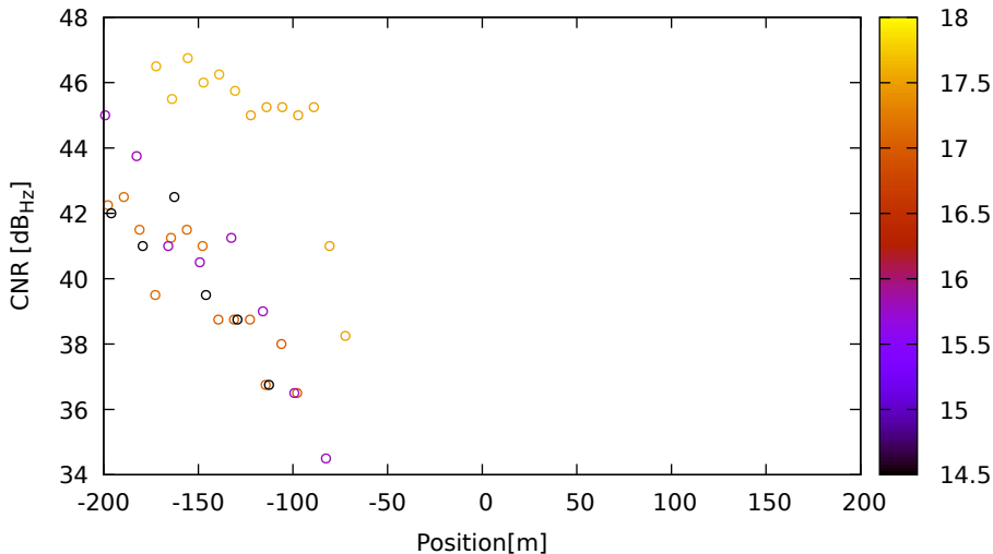
CNR vs position for E04 (E1) on LeicaGS15 - DOY 262 jam. 2
