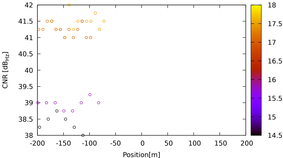
CNR vs position for E04 (E5a) on LeicaGS15 - DOY 262 jam. 2
