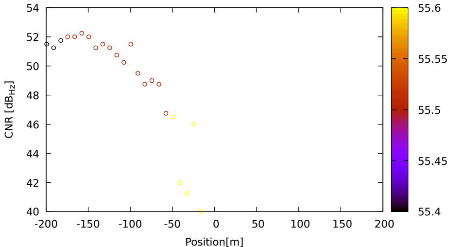
CNR vs position for E05 (E1) on LeicaGS15 - DOY 262 jam. 3
