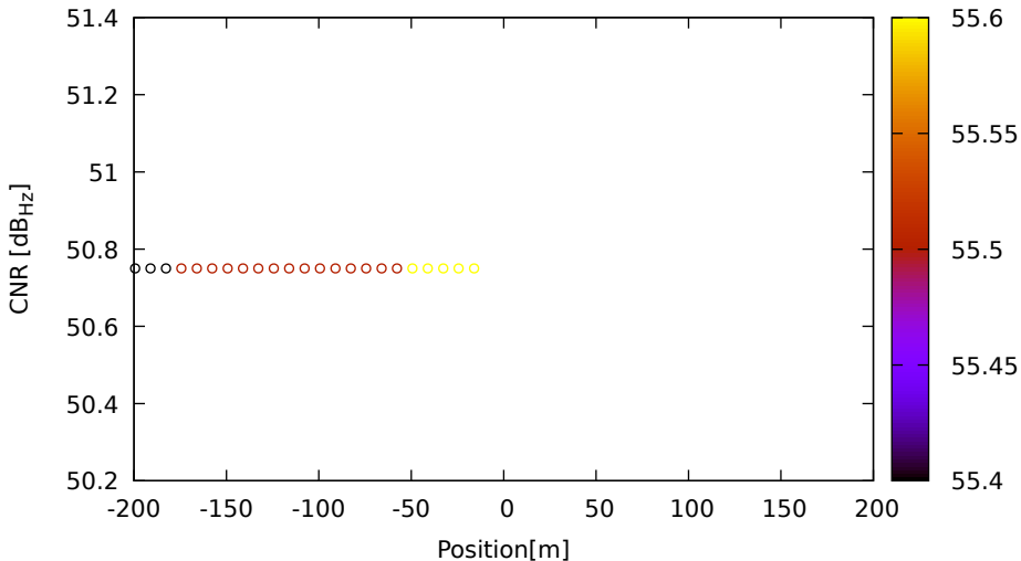
CNR vs position for E05 (E5b) on LeicaGS15 - DOY 262 jam. 3
