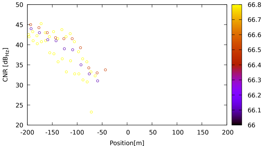
CNR vs position for E09 (E5) on LeicaGS15 - DOY 262 jam. 1
