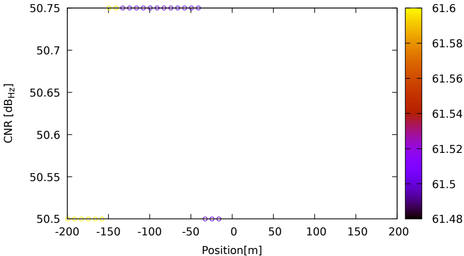
CNR vs position for E09 (E5b) on LeicaGS15 - DOY 262 jam. 3
