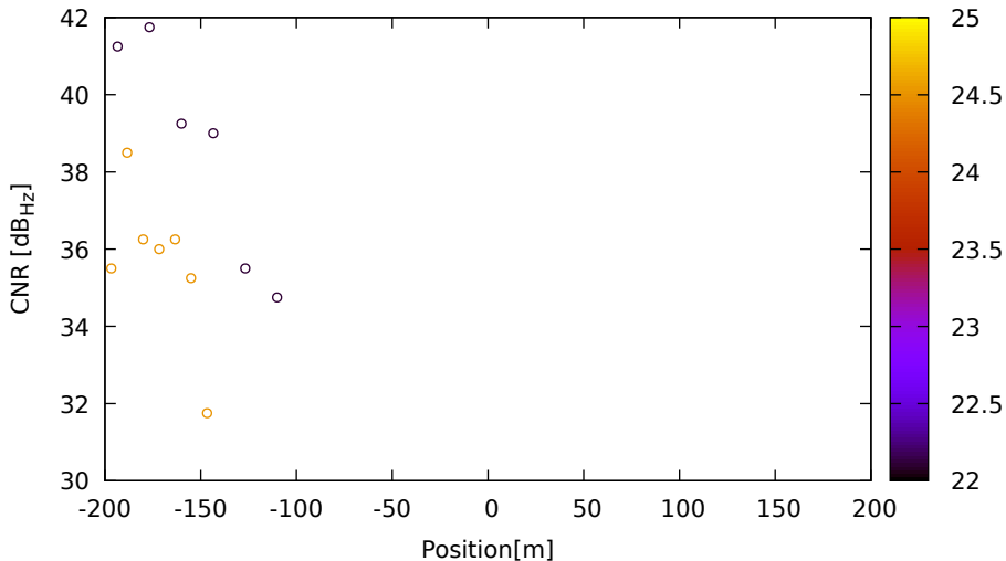
CNR vs position for E11 (E1) on LeicaGS15 - DOY 262 jam. 1
