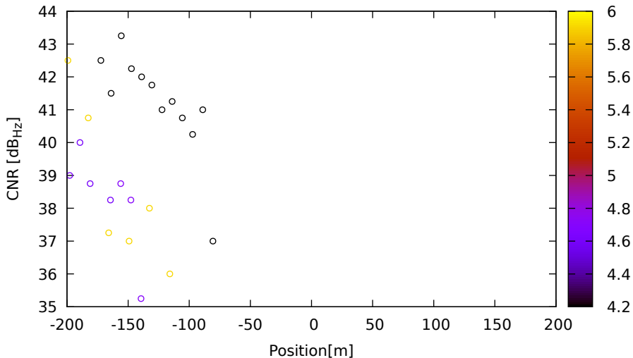
CNR vs position for E15 (E1) on LeicaGS15 - DOY 262 jam. 2
