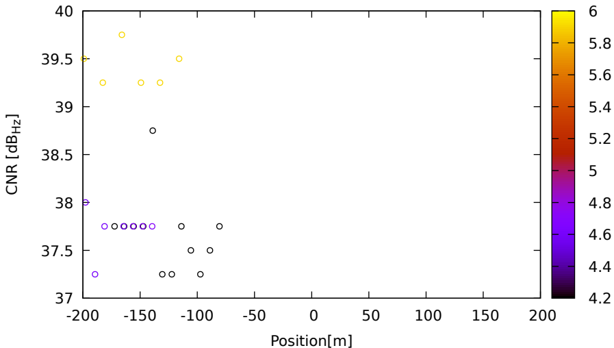
CNR vs position for E15 (E5a) on LeicaGS15 - DOY 262 jam. 2
