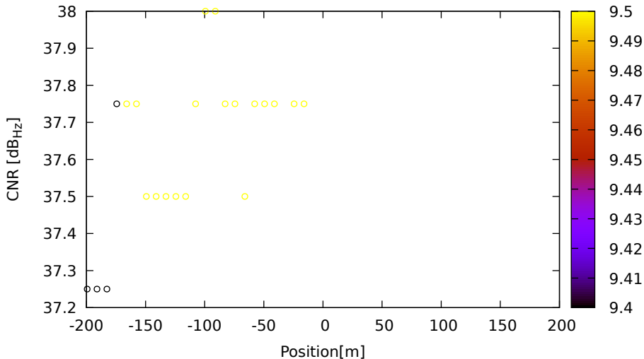
CNR vs position for E15 (E5a) on LeicaGS15 - DOY 262 jam. 3
