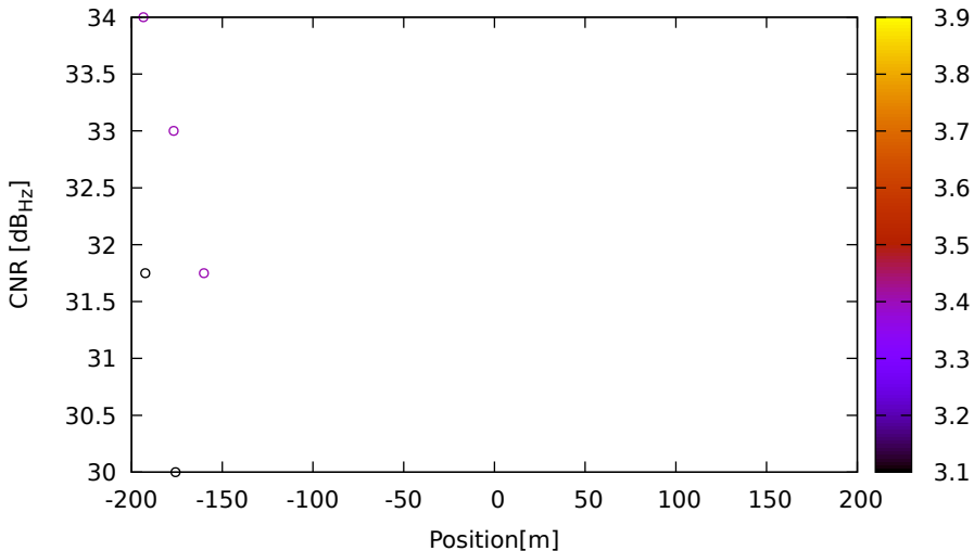
CNR vs position for E27 (E5) on LeicaGS15 - DOY 262 jam. 1
