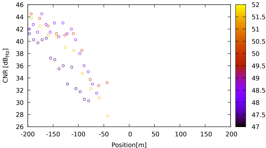
CNR vs position for E34 (E5) on LeicaGS15 - DOY 262 jam. 1
