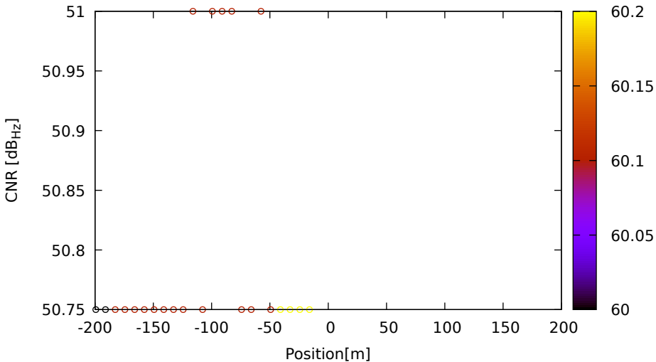
CNR vs position for E34 (E5b) on LeicaGS15 - DOY 262 jam. 3
