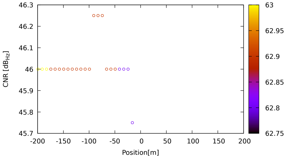
CNR vs position for E36 (E5) on LeicaGS15 - DOY 262 jam. 3
