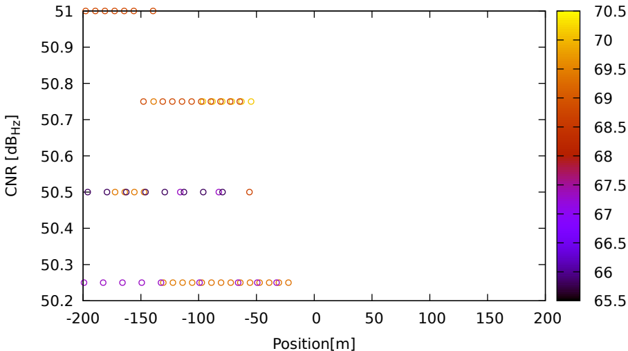
CNR vs position for E36 (E5b) on LeicaGS15 - DOY 262 jam. 2
