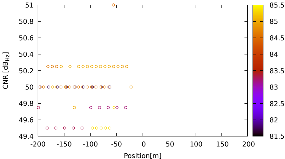
CNR vs position for G01 (L5) on LeicaGS15 - DOY 262 jam. 2
