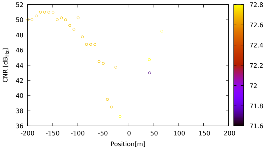
CNR vs position for G03 (L1) on LeicaGS15 - DOY 262 jam. 3
