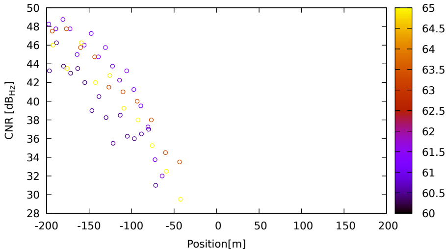
CNR vs position for G03 (L2) on LeicaGS15 - DOY 262 jam. 1
