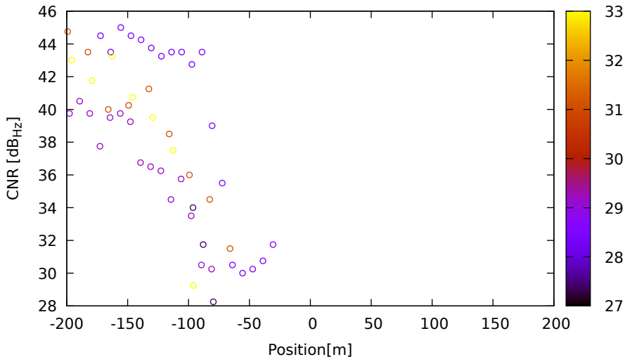
CNR vs position for G04 (L1) on LeicaGS15 - DOY 262 jam. 2
