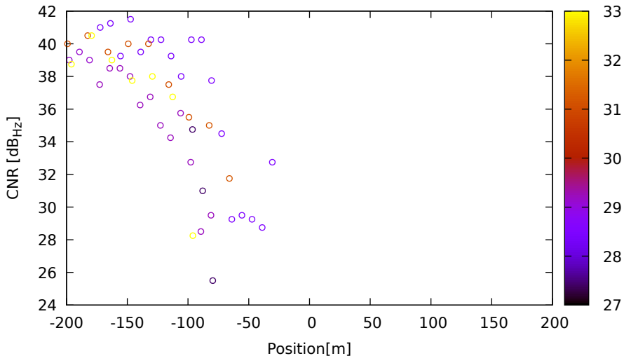
CNR vs position for G04 (L2) on LeicaGS15 - DOY 262 jam. 2
