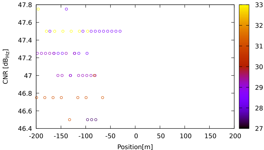
CNR vs position for G04 (L5) on LeicaGS15 - DOY 262 jam. 2
