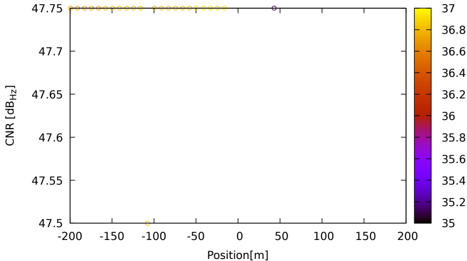
CNR vs position for G04 (L5) on LeicaGS15 - DOY 262 jam. 3
