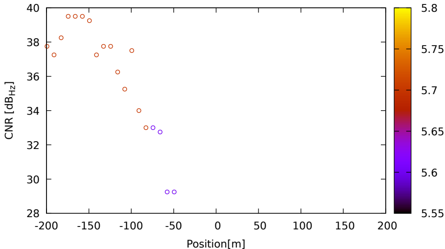
CNR vs position for G08 (L1) on LeicaGS15 - DOY 262 jam. 3
