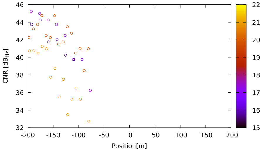
CNR vs position for G08 (L5) on LeicaGS15 - DOY 262 jam. 1
