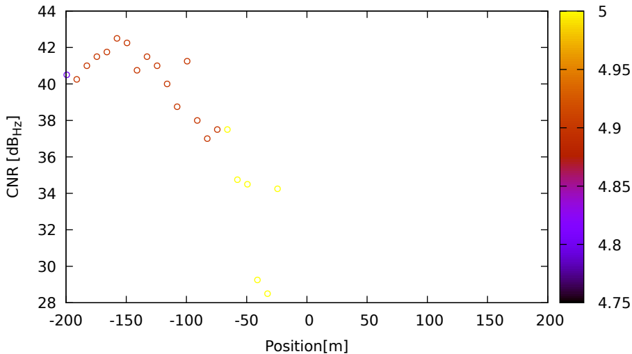
CNR vs position for G09 (L1) on LeicaGS15 - DOY 262 jam. 3
