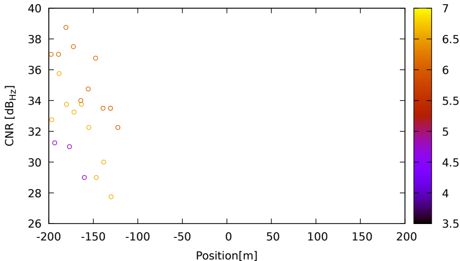
CNR vs position for G14 (L1) on LeicaGS15 - DOY 262 jam. 1
