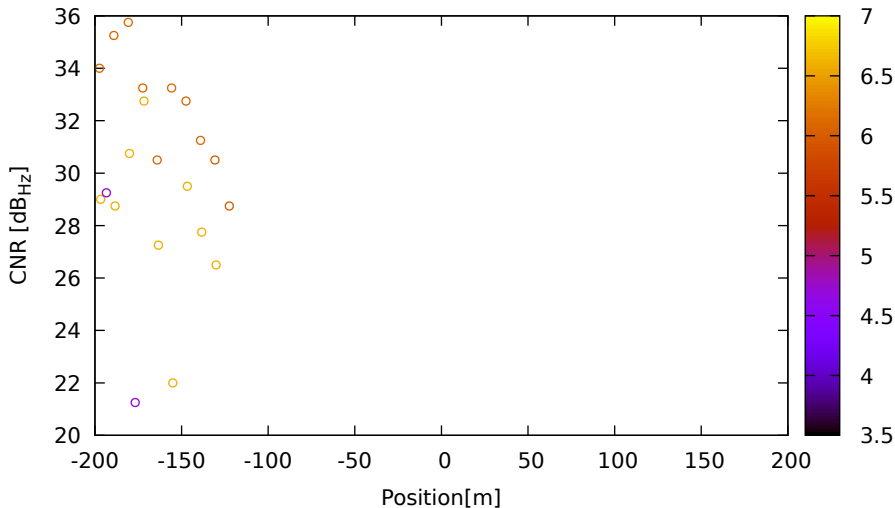
CNR vs position for G14 (L2) on LeicaGS15 - DOY 262 jam. 1
