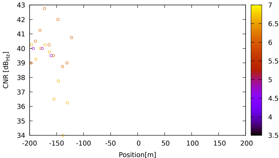
CNR vs position for G14 (L5) on LeicaGS15 - DOY 262 jam. 1
