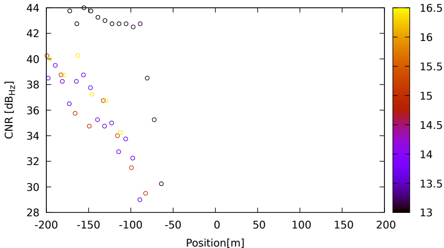
CNR vs position for G19 (L1) on LeicaGS15 - DOY 262 jam. 2
