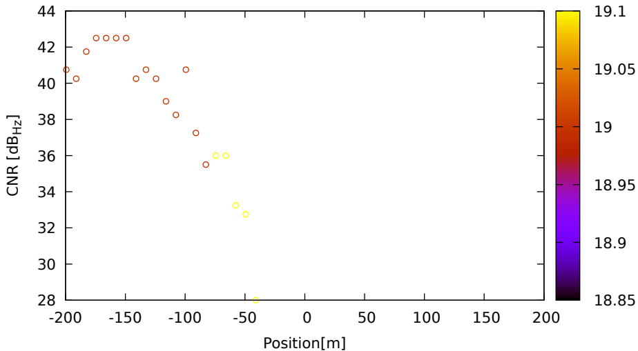
CNR vs position for G19 (L1) on LeicaGS15 - DOY 262 jam. 3
