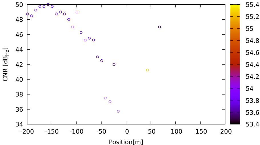
CNR vs position for G21 (L1) on LeicaGS15 - DOY 262 jam. 3
