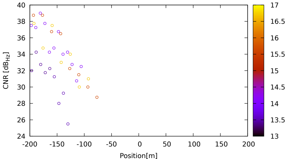
CNR vs position for G31 (L1) on LeicaGS15 - DOY 262 jam. 1
