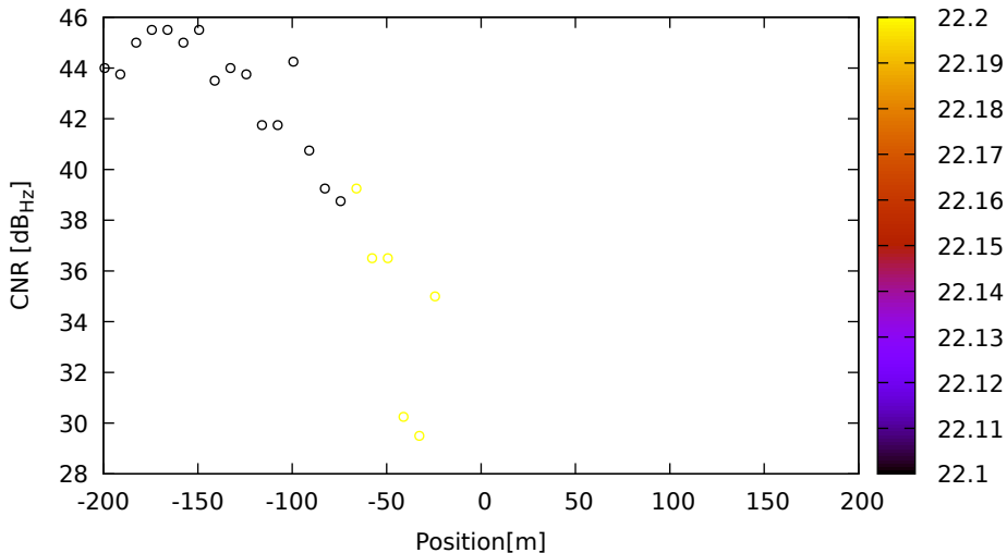
CNR vs position for G31 (L2) on LeicaGS15 - DOY 262 jam. 3
