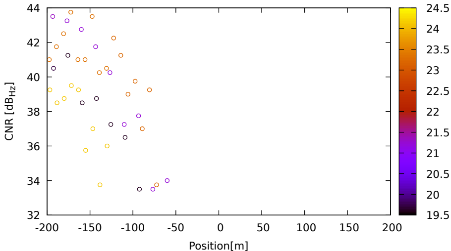
CNR vs position for G32 (L5) on LeicaGS15 - DOY 262 jam. 1
