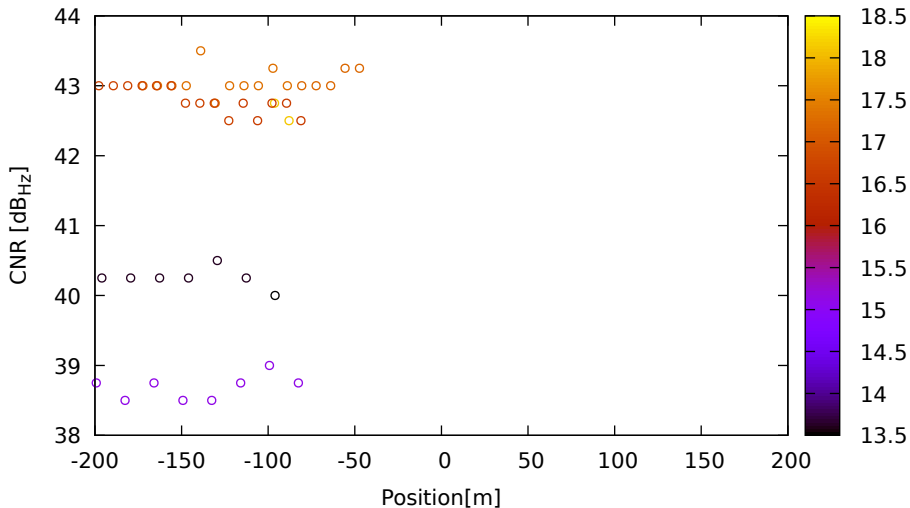
CNR vs position for G32 (L5) on LeicaGS15 - DOY 262 jam. 2
