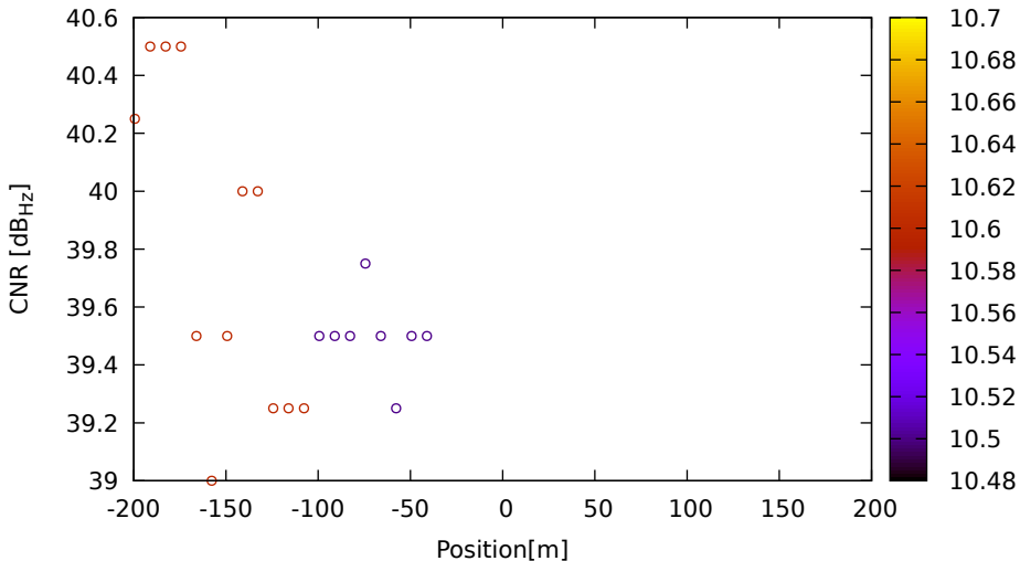
CNR vs position for G32 (L5) on LeicaGS15 - DOY 262 jam. 3
